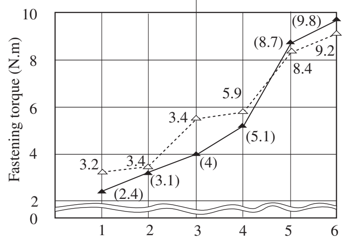
The relation of indication on torque adjusting ring and torque of clutch disengaging
